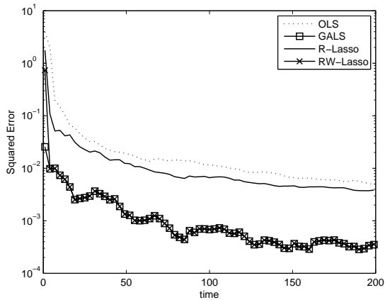
Fig. 1. Squared estimation error when \mathbf{x} is time-invariant.
