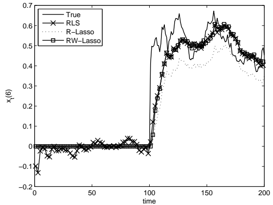
Fig. 4. Time evolution of the x_6 signal entry.
